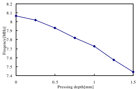
Fig. 11: Oscillating frequency vs. pressing depth.
