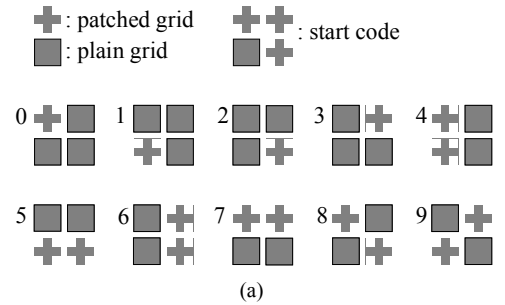
Figure 2. (a) is the normal mesh pattern for 2DST sheet. (b) is the example of position coding mesh pattern. The patched grid has four square patches on the corners, and we express 1 bit information by whether the grid has the patches or not.
