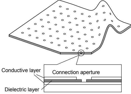
Figure 1 Schematic illustration of TDC sheet.
