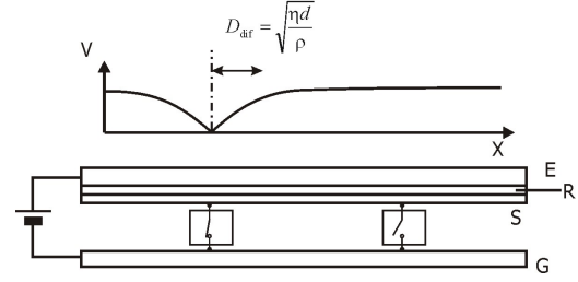
Fig. 3: Illustration of diffusive signal transmission in type I. A signal sent from a chip is detected only by chips inside the D_{\text{dif}} circle.
