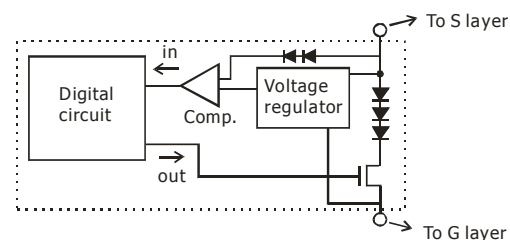
Fig. 8: The structure of the communication chip for Type I architecture.
