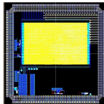
Fig. 9: The mask pattern we designed for a 1st-order communication chip. The chip size is 5 mm by 5mm with digital circuit of 3 mm by 2mm.
